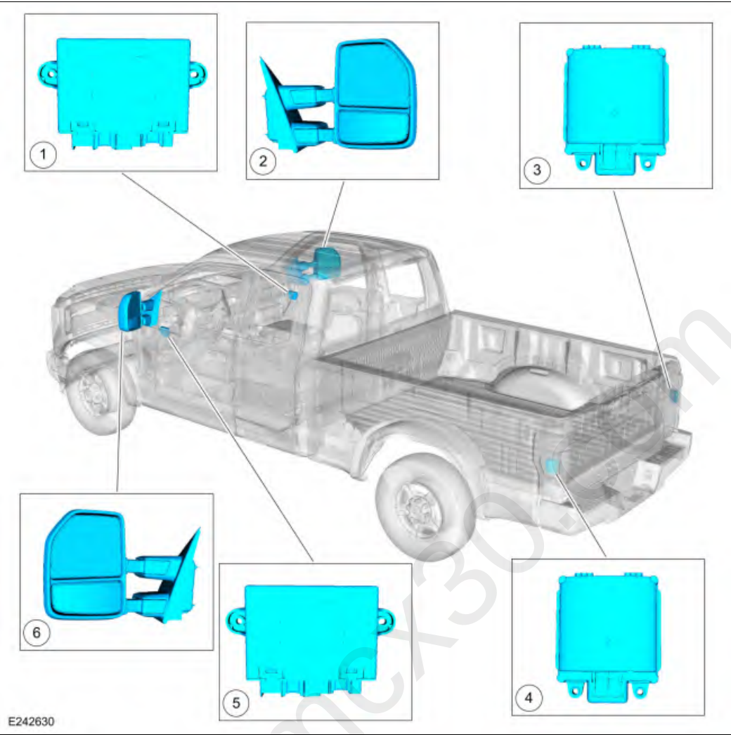
Component Location - Blind Spot Monitoring System (BLISÂ®)
